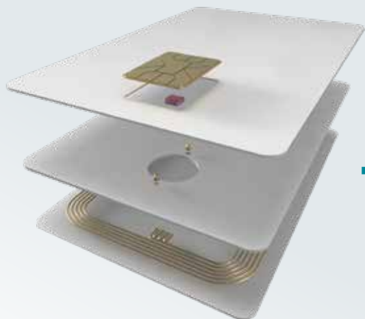
SCI 202 Fully-Automatic Implanting of IC Modules into Plastic Cards
